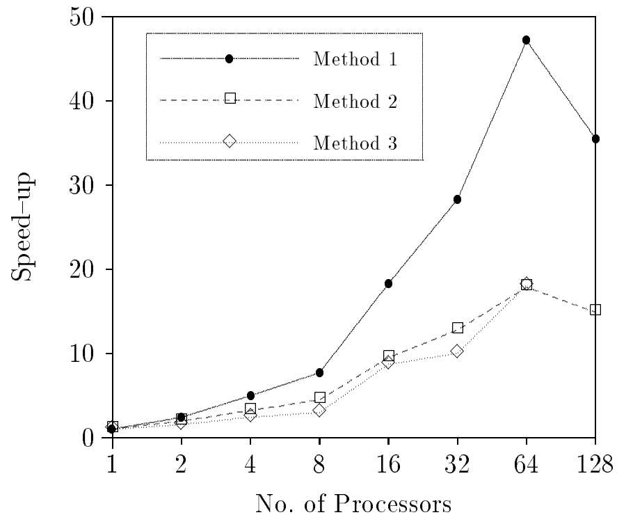
Speed-up for parallelization method 1-3 for the 1st test case.
