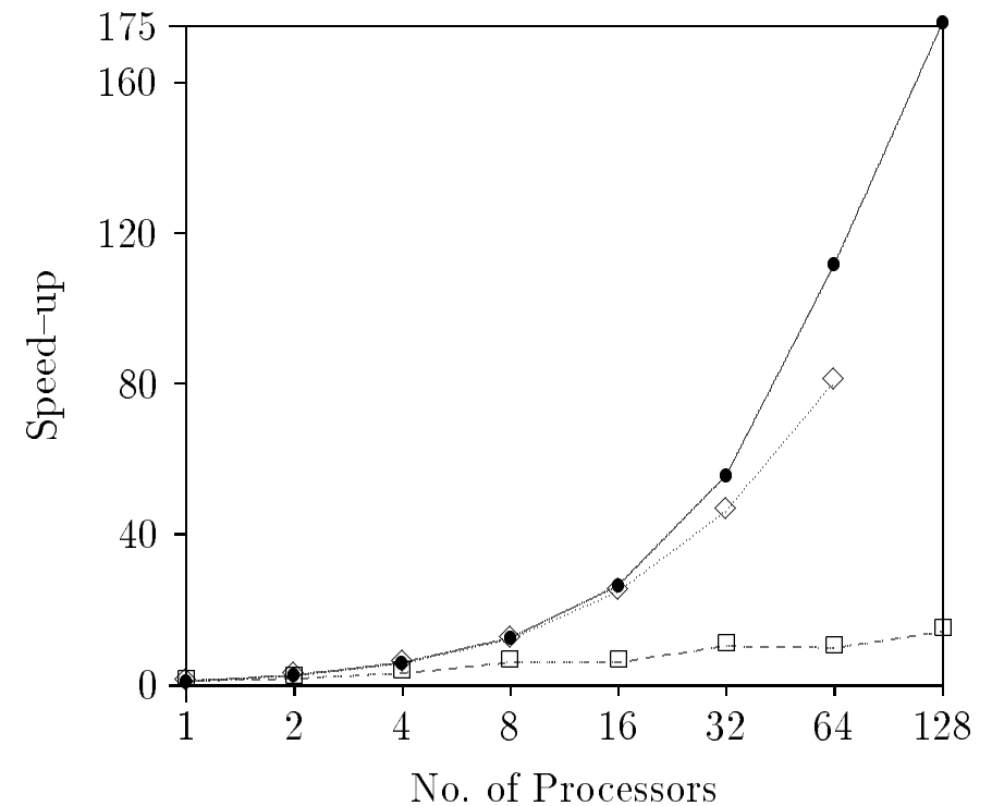
Speed-up for parallelization method 1-3 for the 2nd test case.
