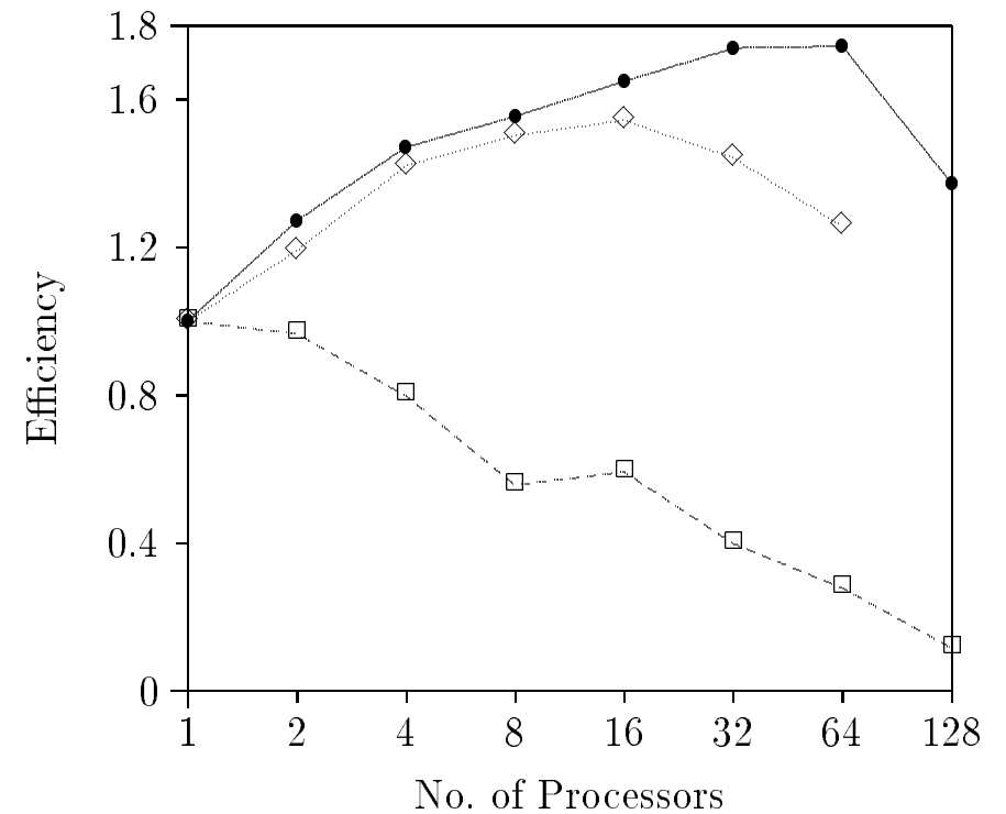
Efficiency for parallelization method 1-3 for the 2nd test case.
