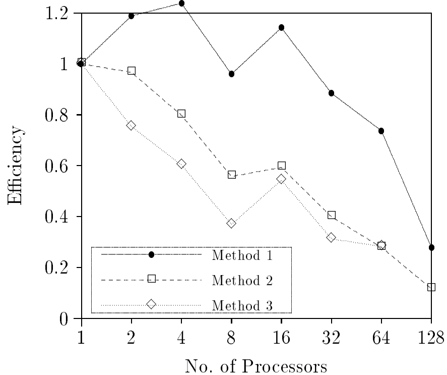
Efficiency for parallelization method 1-3 for the 1st test case.
