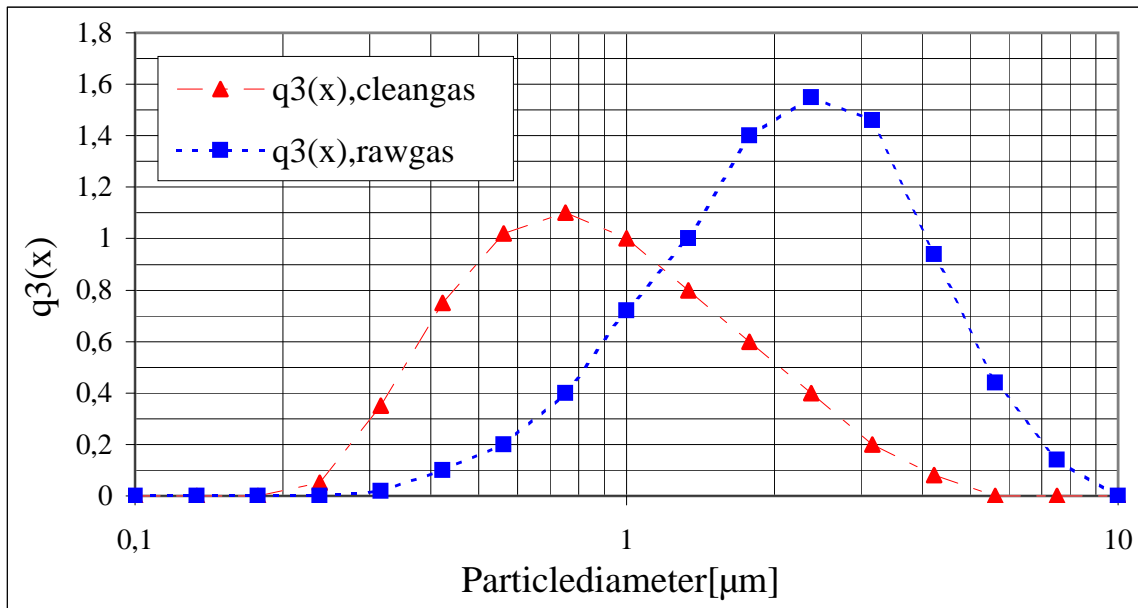
Frequency distribution q_3(x) based on particle volume for cyclone ZT30.
