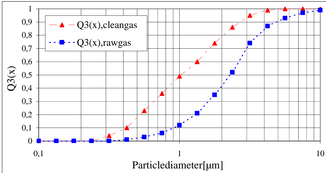
Cumulative distribution function Q_3(x) based on particle volume for cyclone ZT30.
